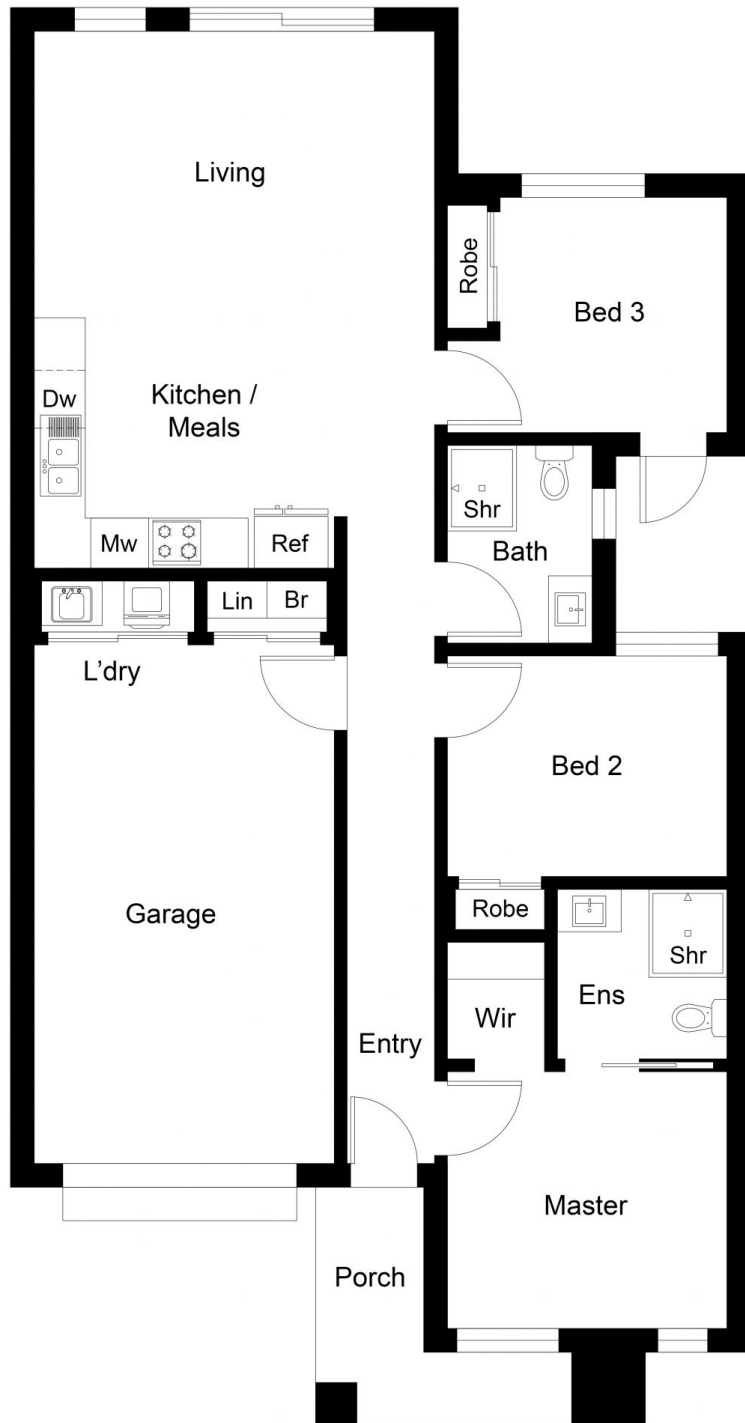
FLOOR PLAN
